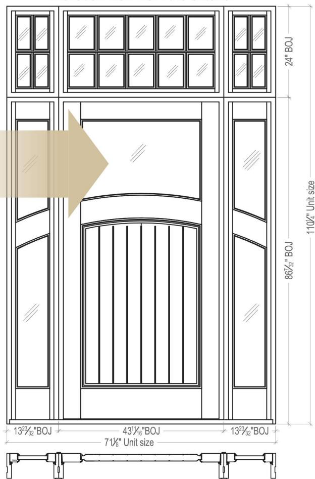
Elevation view from the exterior
